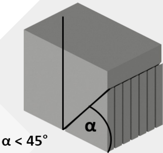
Figure 5: Overhang Angle
